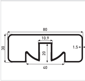
1,147 kg/m ER.8221
